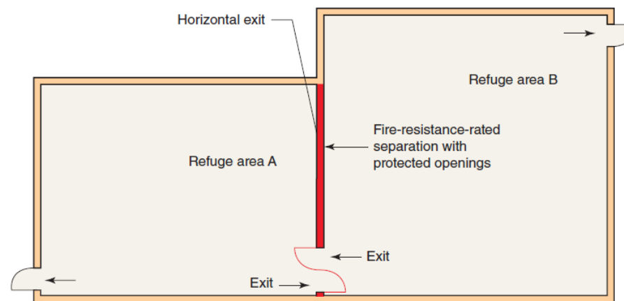
Horizontal exits
